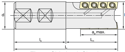
Fig. 1: Side Lock Shank
